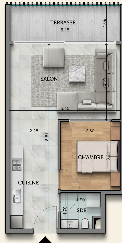
Type 2 57m 2
